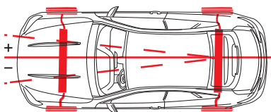
Positive & Negative Thrust Angle
